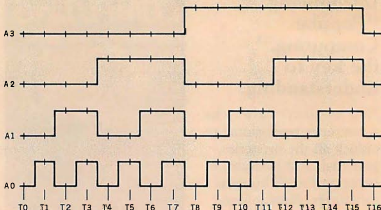
TIMING DIAGRAM
