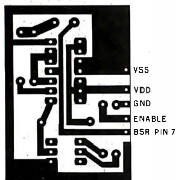
Figure 2: Interface etching, drilling, and component layout. A printed-circuit card of the proper size (the figure is actual size) will fit easily in the controller's case, although other construction techniques may work as well. Note the orientation of pin 1 on each of the integrated circuits.
